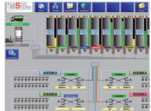
Silo loading
