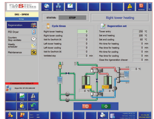
Dryer
